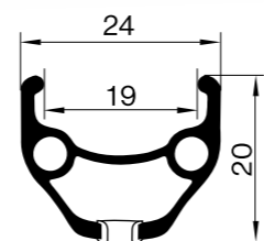
TOP DISC - RX 3019 26" 498 g | 27,5" 512 g | 29" 554 g
