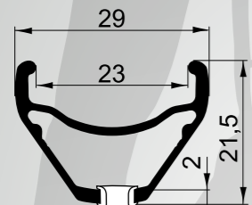
WER - RX 2023 26" 514 g | 27,5" 542 g | 29" 578 g
