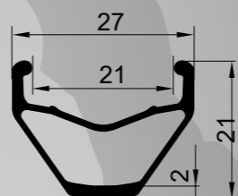
HURRY - RX 2021 26" 468 g | 27,5" 496 g | 29" 524 g
