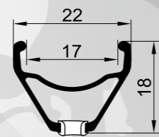
XCO RIO - RX 2017 26" 392 g | 27,5" 418 g | 29" 442 g
