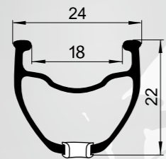
FAST DISC - RX 2018 26" 496 g | 27,5" 514 g | 29" 546 g
