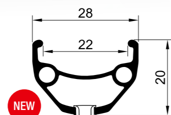
ROCKY 22 - RX 3022 26" 562 g | 27,5" 587 g | 29" 625 g
