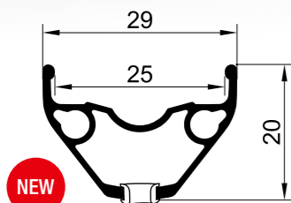
E-ROCKY - RX 3025 26" 558 g | 27,5" 583 g | 29" 621 g
