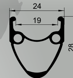
GRAND ROCK - RX 3019 26" 614 g | 29" 680 g
