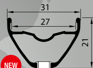
ENDURO - RX 2027 27,5" 474 g | 29" 502 g
