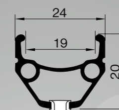
DRAGON LINE - RX 719 20" 350 g | 26" 500 g 27,5" 540 g | 29" 582 g
