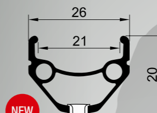
HIT 21 - RX 4521 26" 527 g | 27,5" 550 g | 29" 586 g
